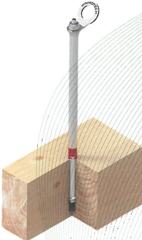
Fig. 1: Anchor device type A, type POINT-11
